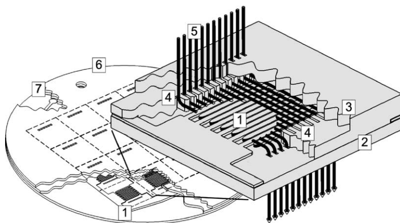
Fig. 1. Scheme of the multireactor, microreactor single cell and gas flow (numbered features explained in text).
