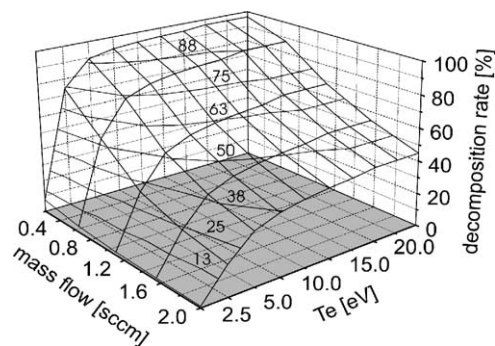
Fig. 2. Decomposition rates resulting from CFD simulation.
